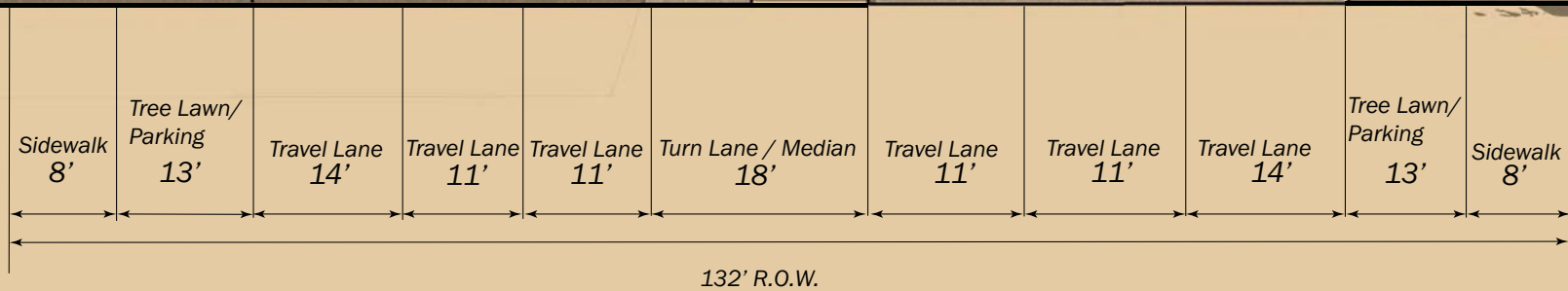
46th Avenue Concept Cross Section Elyria Swansea Small Area Plan 10.29.2008
